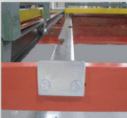
Notched rails allow easy cart access while eliminating lift out and derailing
